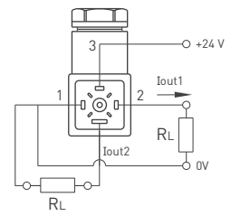
0-20mA and 4-20mA Output
