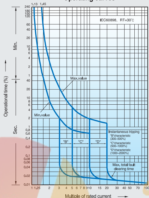
Operating curves
