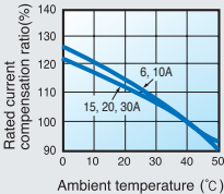
Compensation curves
