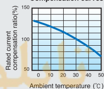
Compensation curves
