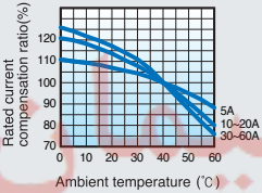
Temperature curve
