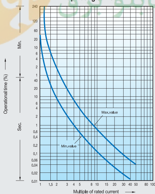
Operating curves
