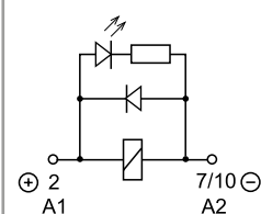
C: Option 6, 7, 74 LED + diode (DC, polarity positive to pin 2)
