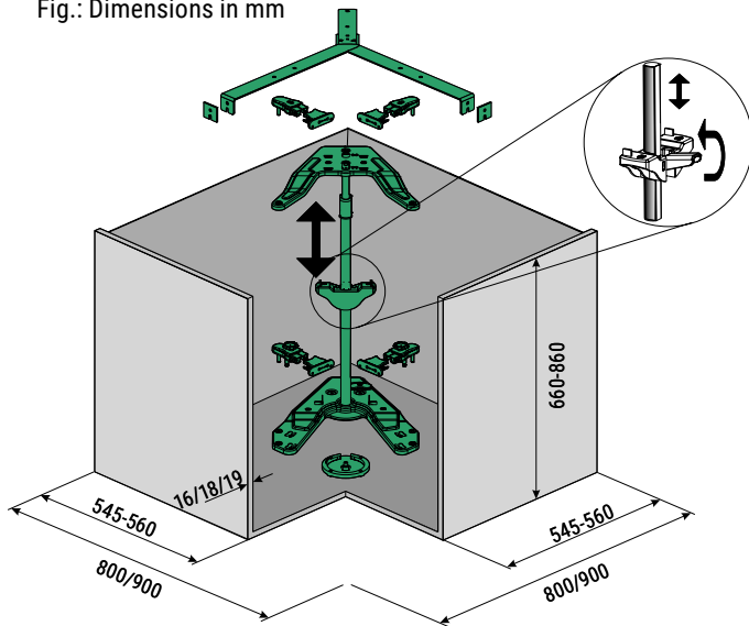
Fig.: Dimensions in mm
