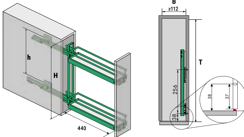
Fig.: Dimensions in mm
