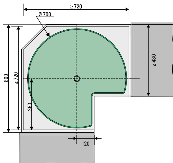
Fig.: Dimensions in mm
