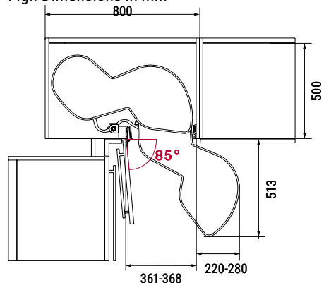
Example: swings out to the right (left cabinet – 40 cm door)
