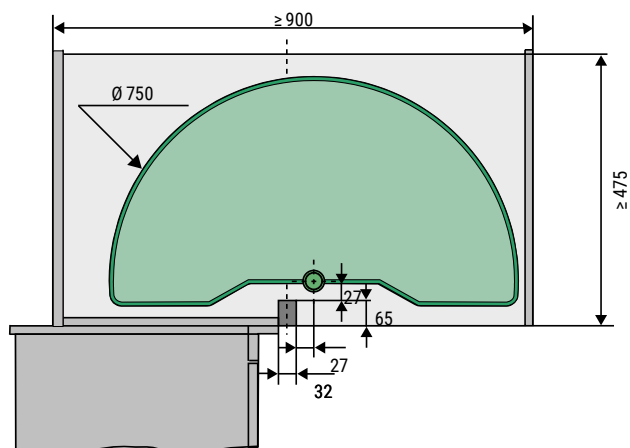
Fig.: Dimensions in mm
