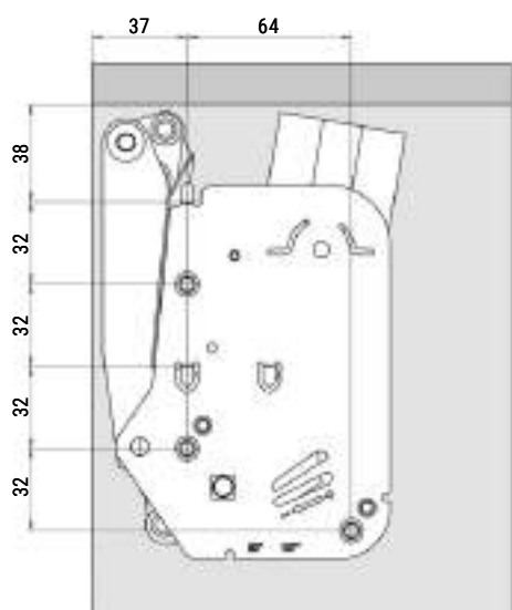
View from right (left fitting)
