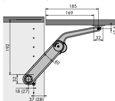
View left carcass side (lifter installed right)
