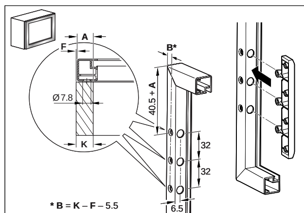
Front connectors for 20 mm aluminium frames
