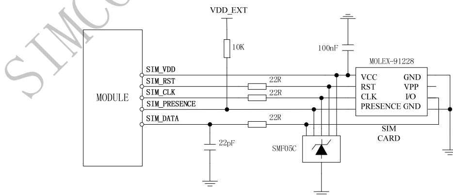
Figure 28: Reference circuit of the 8-pin SIM card holder
