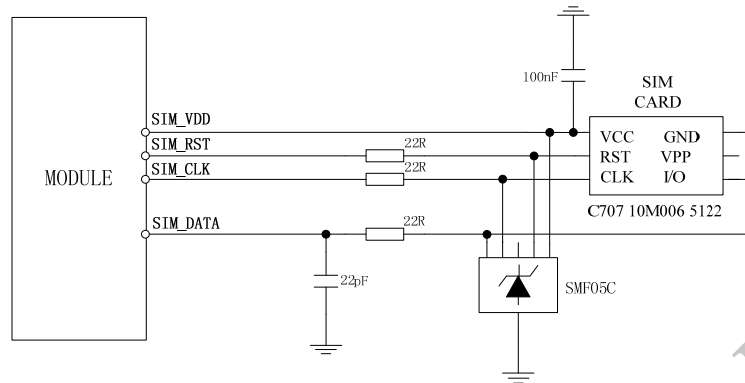
Figure 29: Reference circuit of the 6-pin SIM card holder
