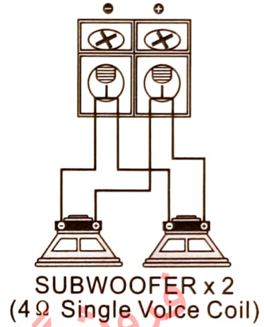
2 Ohms Load
