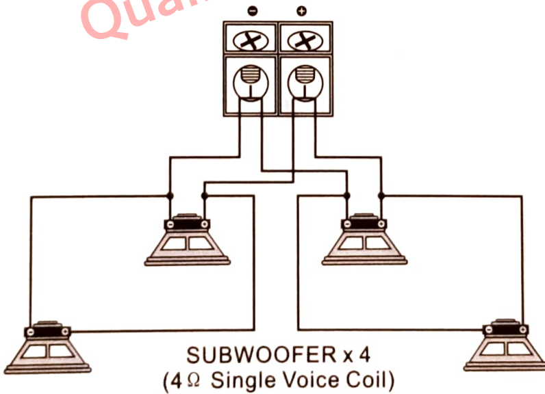
1 Ohm Load
