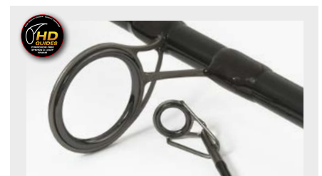
Light and strong double leg HD SIC guides, with 40 mm size on butt section.
