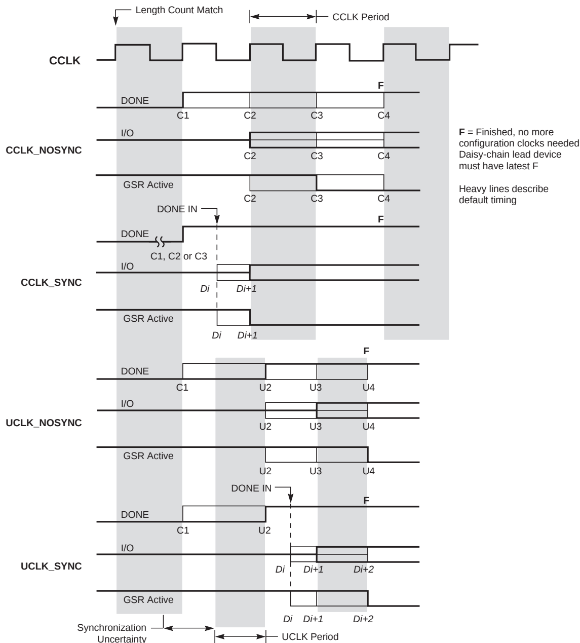
Figure 31: Start-up Timing
