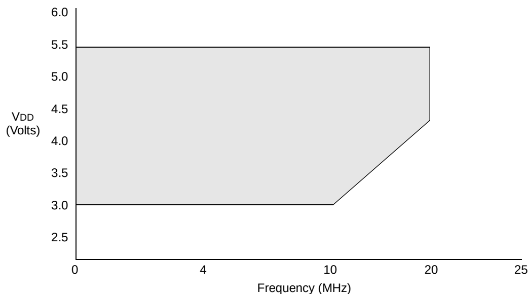
FIGURE 15-1: PIC16C54C VOLTAGE-FREQUENCY GRAPH, 0^{\circ}\text{C} \leq T_A \leq +70^{\circ}\text{C}
