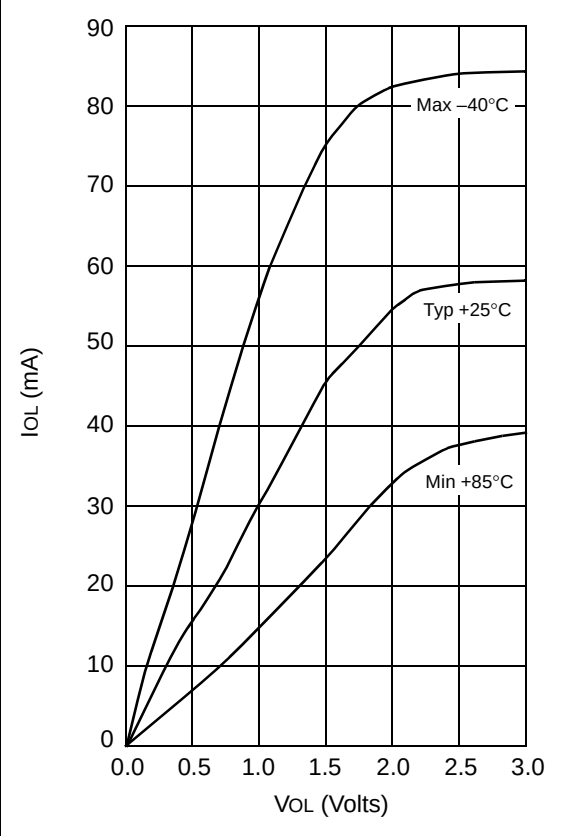
FIGURE 14-22: I_{OL} vs. V_{OL} , V_{DD} = 5\text{ V}
