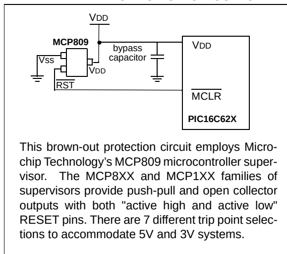
FIGURE 7-16: EXTERNAL BROWN-OUT PROTECTION CIRCUIT 3
