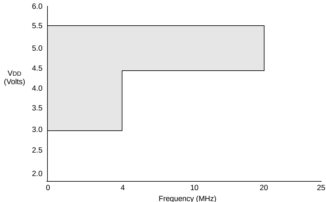
FIGURE 15-2: PIC16C54C VOLTAGE-FREQUENCY GRAPH, -40^{\circ}\text{C} \leq T_A < 0^{\circ}\text{C} , +70^{\circ}\text{C} < T_A \leq +125^{\circ}\text{C}
