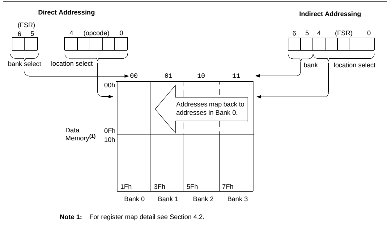
FIGURE 4-10: DIRECT/INDIRECT ADDRESSING
