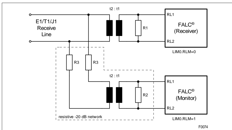
Figure 43 Receive Line Monitoring
