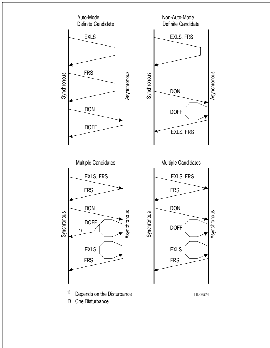
Figure 49 Influences on Synchronization Status (T1/J1)
