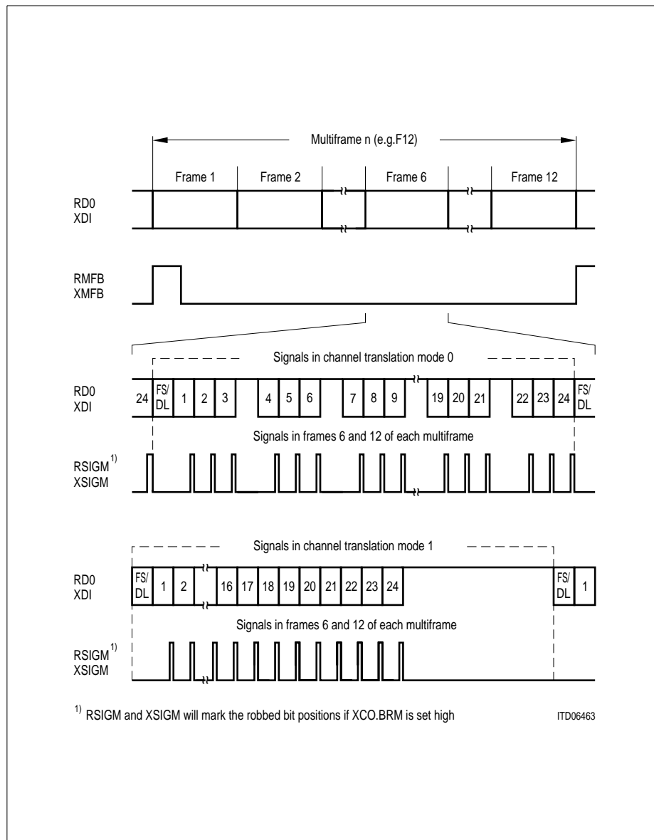
Figure 68 Signaling Marker for CAS-BR Applications (T1/J1)
