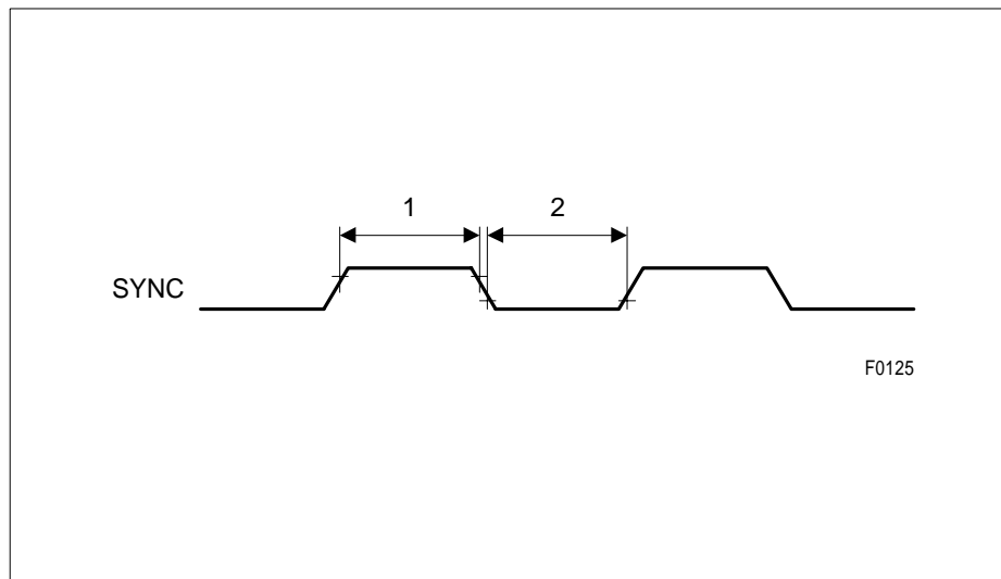
Figure 102 SYNC Timing
