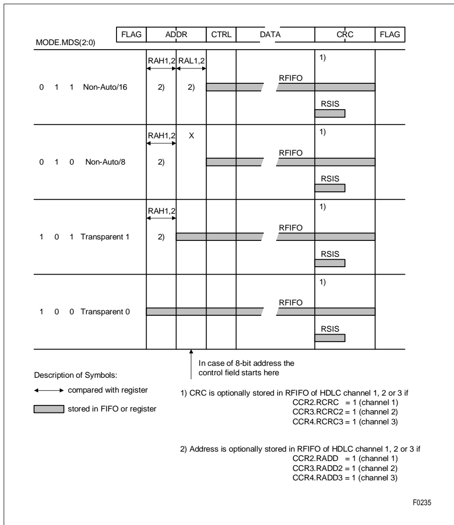
Figure 76 HDLC Receive Data Flow
