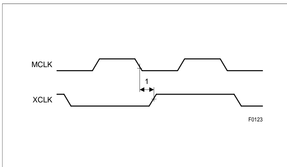
Figure 99 XCLK Timing
