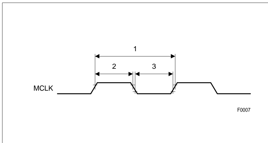
Figure 81 MCLK Timing
