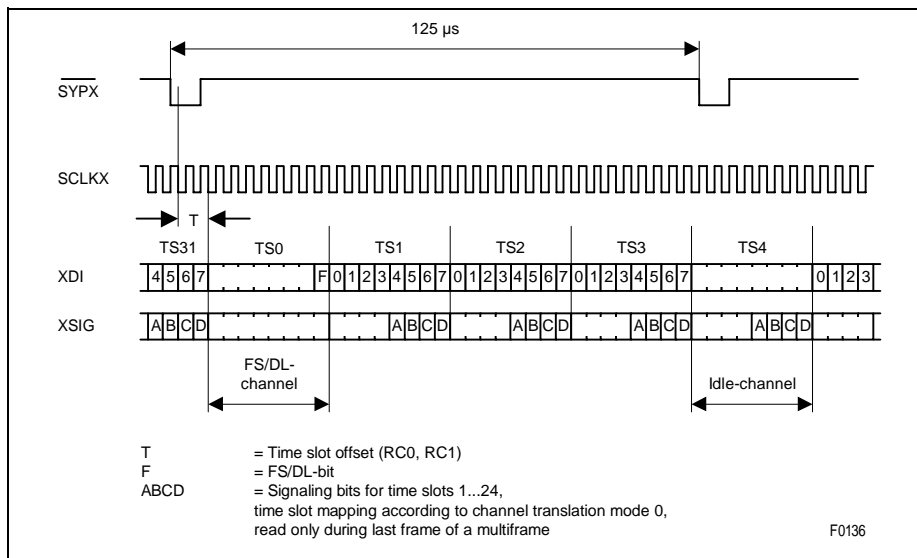
Figure 65 2.048 MHz Transmit Signaling Clocking (T1/J1)
