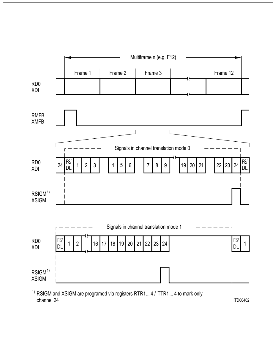
Figure 67 Signaling Marker for CAS/CAS-CC Applications (T1/J1)
