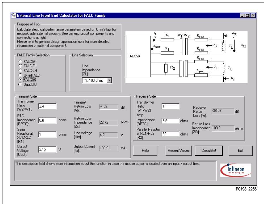
Figure 110 External Line Frontend Calculator
