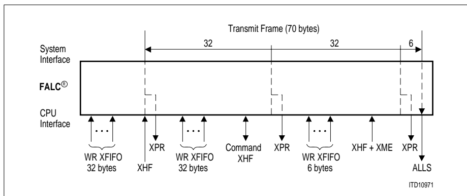
Figure 79 Interrupt Driven Transmission Example
