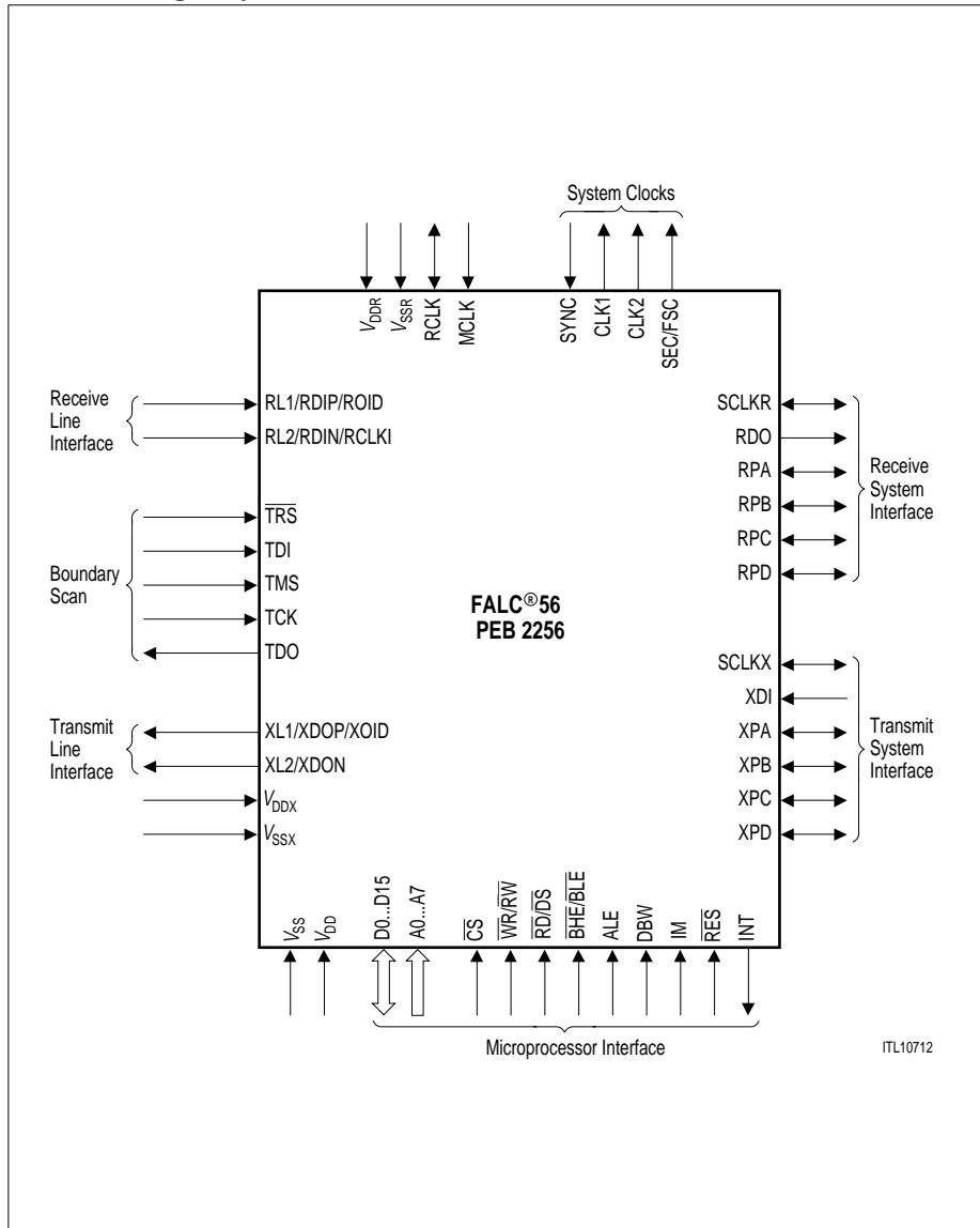
Figure 1 Logic Symbol
