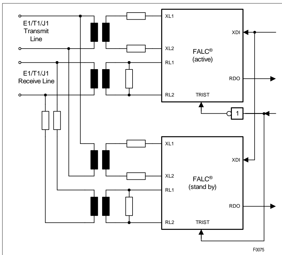
Figure 44 Protection Switching Application
