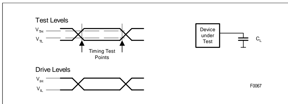
Figure 106 Input/Output Waveforms for AC Testing
