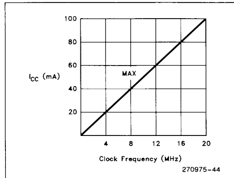
Figure 45. I_{CC} vs Frequency
