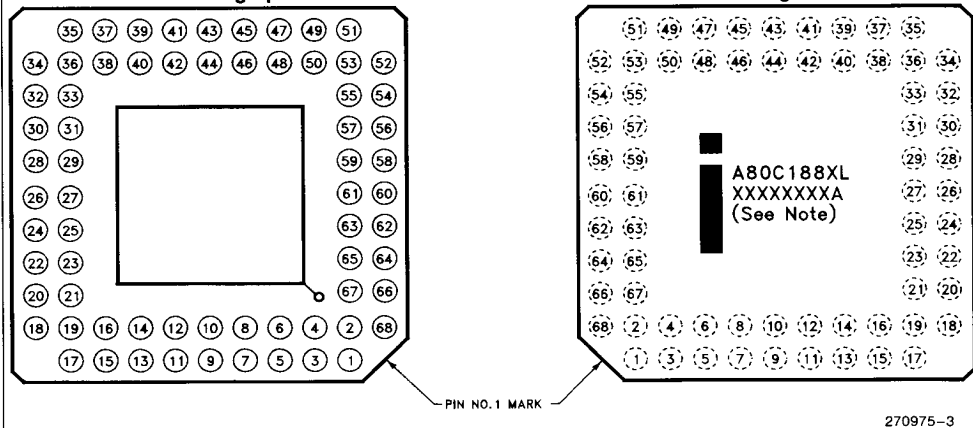
Figure 2. 80C188XL Pinout Diagrams
