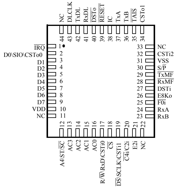
44 PIN QFP
