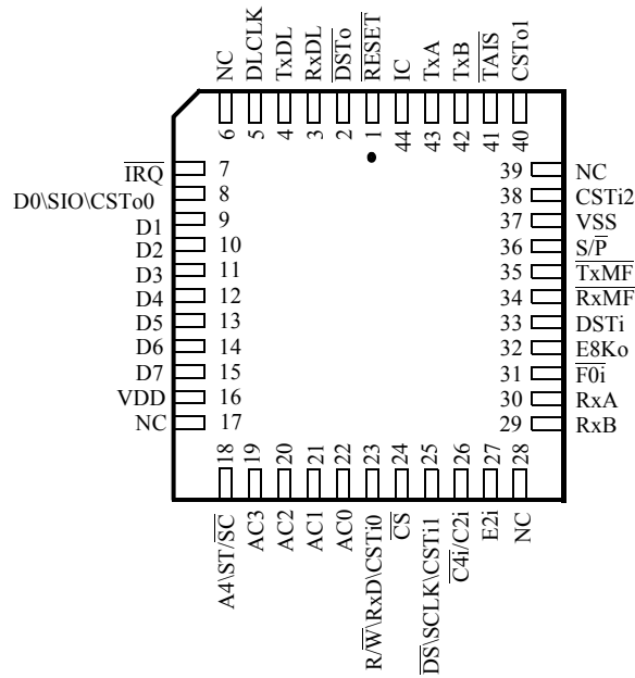
44 PIN PLCC
