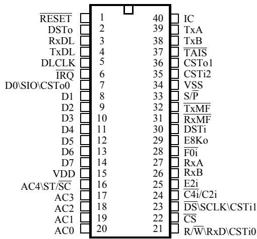
40 PIN PLASTIC DIP
