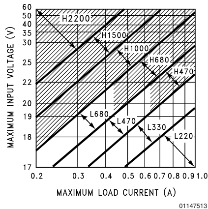
FIGURE 6. LM2575(HV)-15
