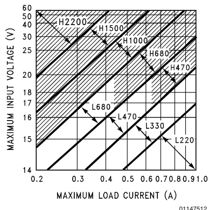
FIGURE 5. LM2575(HV)-12
