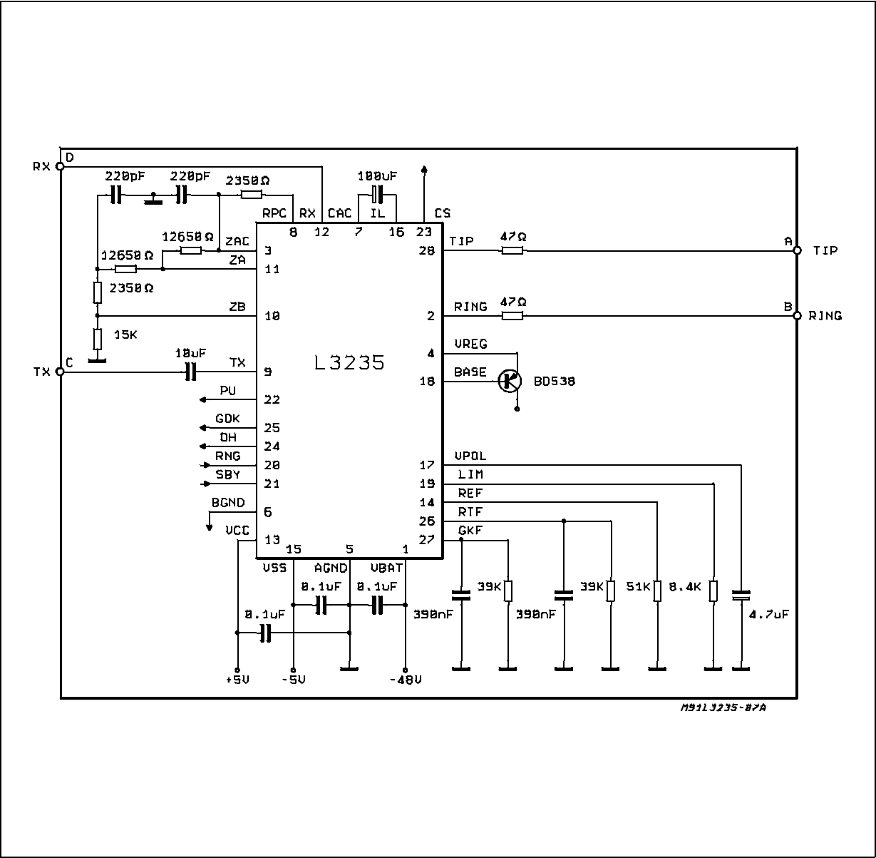
Figure 17: Test Circuit
