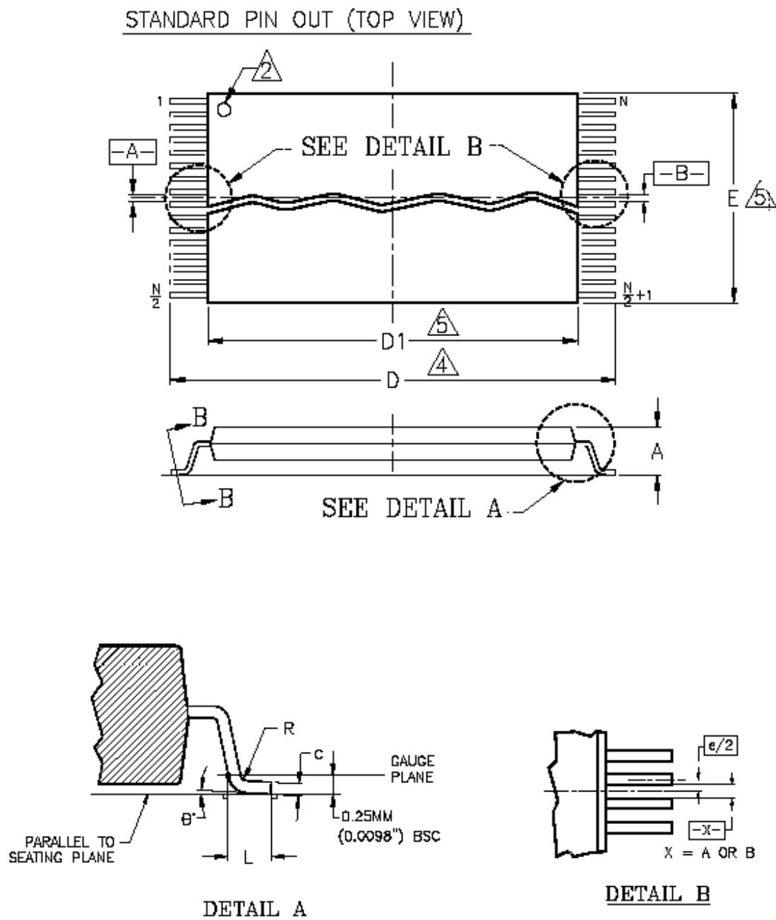
FIGURE 14. TSOP 12mm x 20mm
