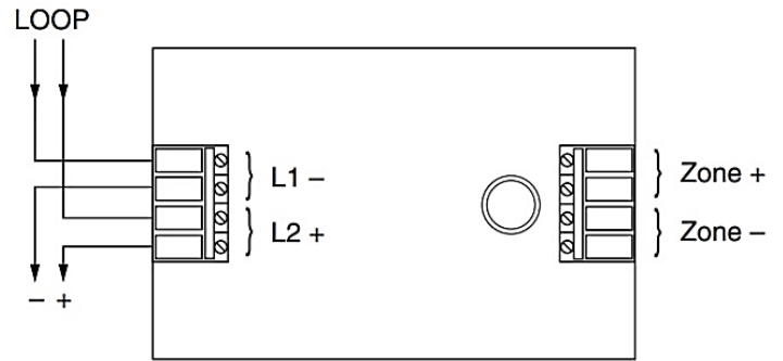
Fig.1 Loop connections
