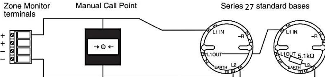
Fig.2 Zone connection — standard bases with 5.1 k \Omega monitoring resistor at end-of-line
