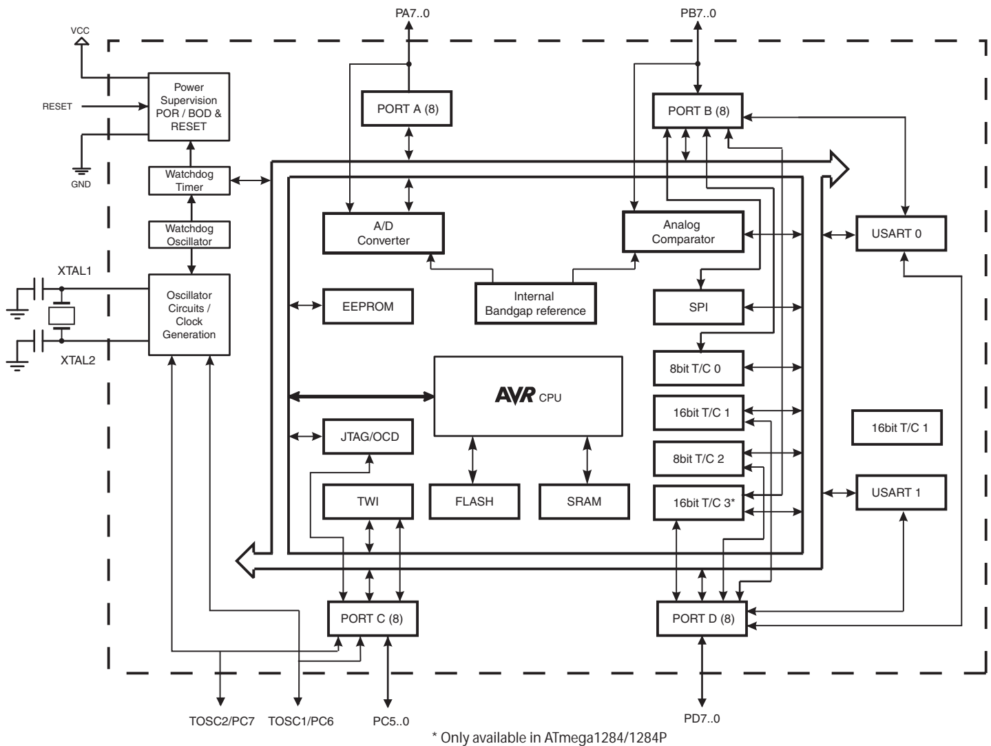
Figure 2-1. Block diagram.
