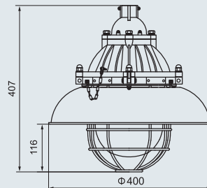
HRD51-250 with external reflector
