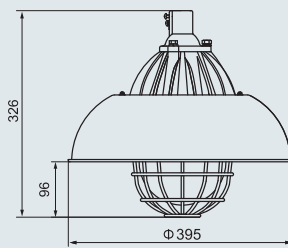
HRD51-150 with external reflector
