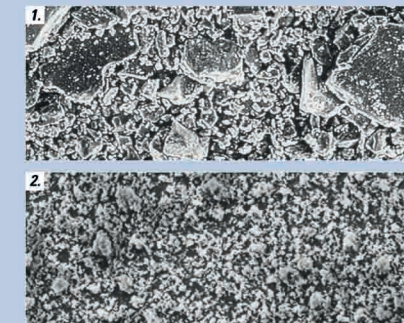
1. Conventional composite: filler photographed at 500x magnification. 2. Saremco microhybrid composite: filler photographed at 500x magnification (the extra low shrinkage is manufactured with the same filler). (Photographs University of Basel)
