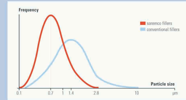
Particle size distribution
