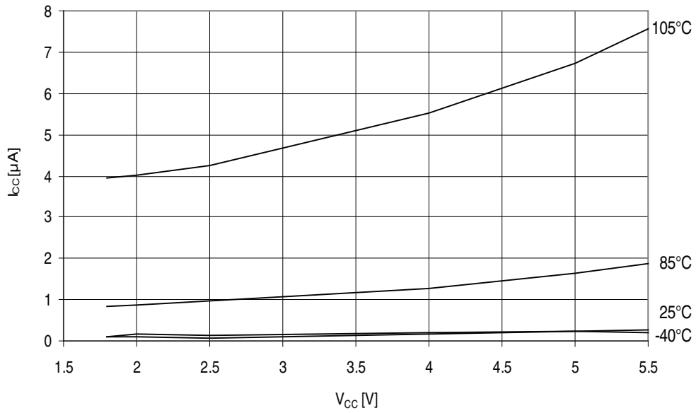
Figure 32-247. ATmega3290A - 105°C: Power-down Supply Current vs. V_{CC} (Watchdog Timer Disabled)
