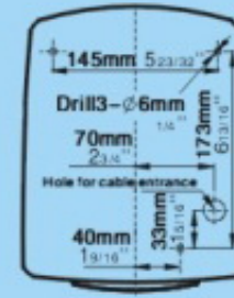
Installation templet
