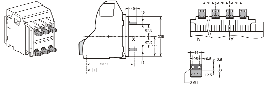
Vertical rear connection
