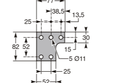
4-pole Left-center or right-center extension terminal
